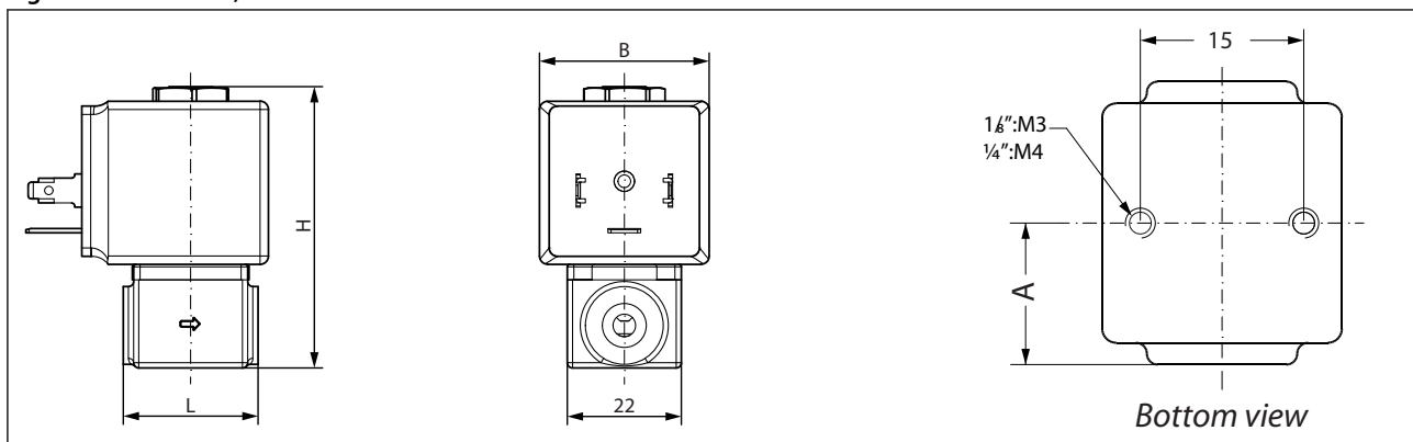
Figure 5: Dimension, brass NC
