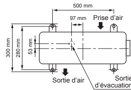
RAS-05, 07, 10, 13E2AVG-E
